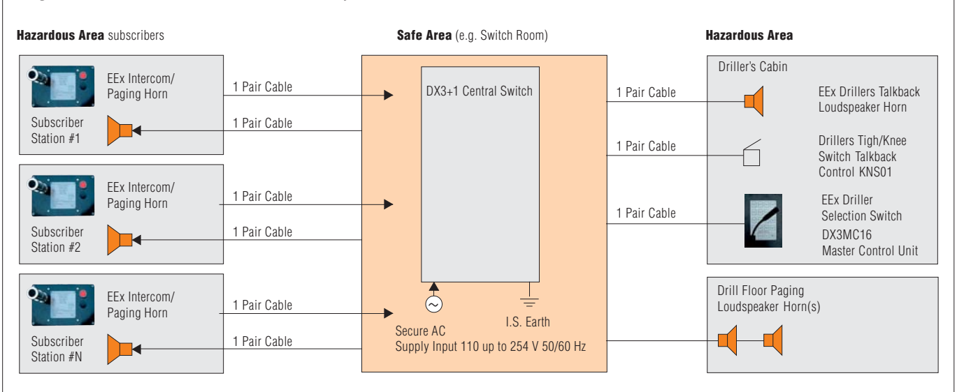
Diagram of Hands-free Drillers Talkback Intercom System
